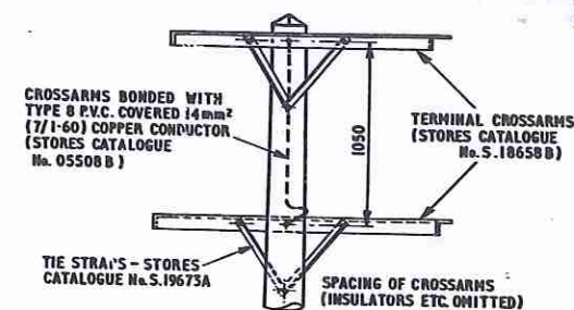
ARRANGEMENT 'C' FOR DEVIATIONS ABOVE 75°
