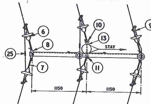
ARRANGEMENT 'A' FOR LINE DEVIATIONS UP TO 30°
