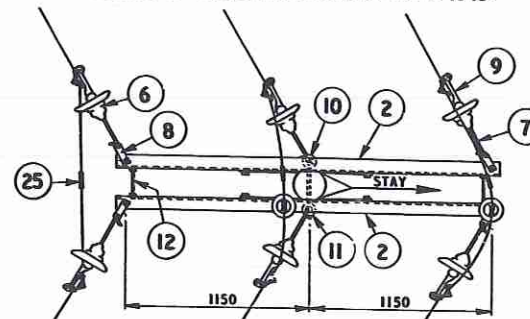
ARRANGEMENT 'B' FOR DEVIATIONS ABOVE 30° AND UP TO 75°
